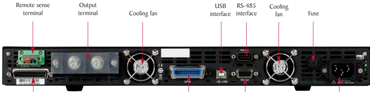
Analog control interface
